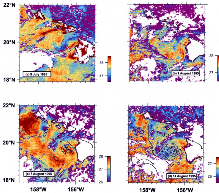
Fig. 2. AVHRR SST images (°C) for (a) 8 July, (b) 1 August–tournament week, (c) 7 August, and (d) 14 August. Concurrent drifter positions (points, with lines showing previous five days) are overlaid SST in (c) and (d). Temperatures colder than 22°C have been flagged as clouds (white).
