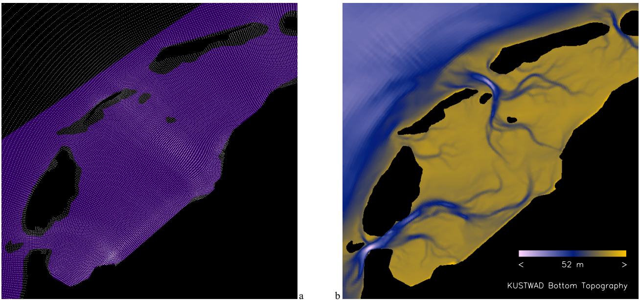
Figure 1. KUSTWAD model grid points and SRTM swath and land mask (a) and KUSTWAD bottom topography (b) in the 70 km × 70 km test area.
